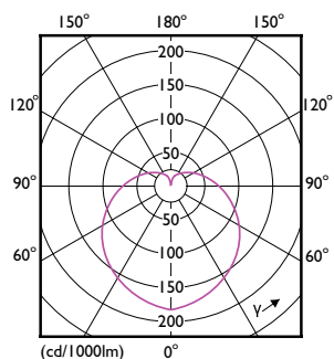
Light Distribution Diagram - PILA LED 40W A60 E27 WW FR ND 1CT/6
