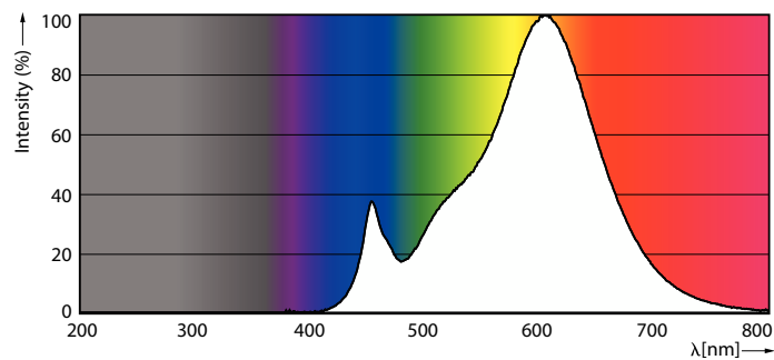
Spectral Power Distribution Colour - PILA LED 40W A60 E27 WW FR ND 1CT/6
