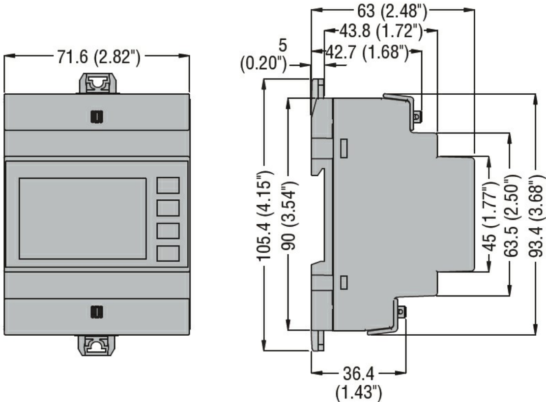
Single-phase
