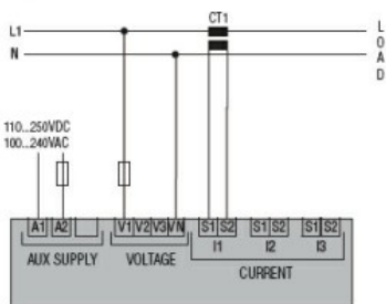
Single-phase
