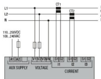
Two-phase
